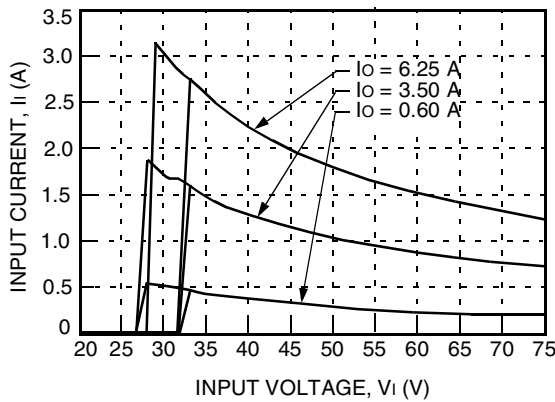
Figure 2. Typical QW075B1 Input Characteristics at Room Temperature
